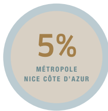
YIELD RATES
